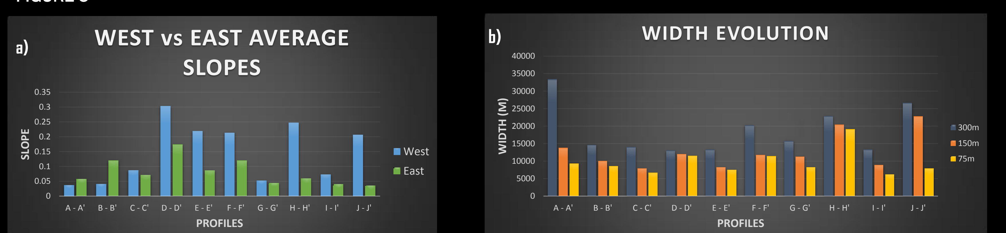
a) Slopes on the west and east sides of the canyon are compared to assess canyon channel symmetry with increasing depths (A-J).
